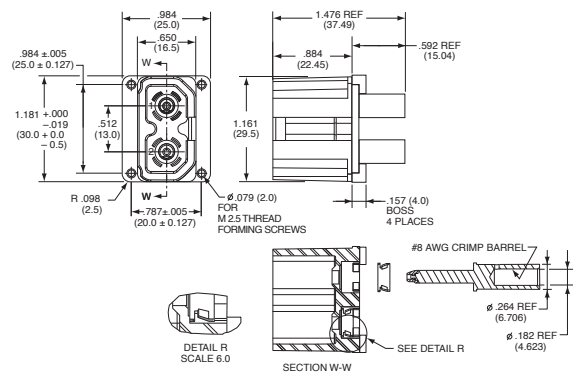
10-638976-000 Busbar Receptacle
