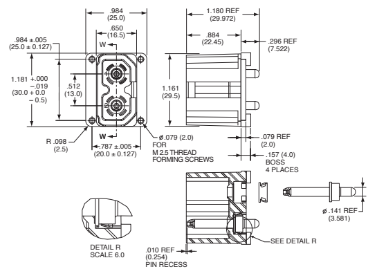
10-638977-000 PCB Tail Receptacle
