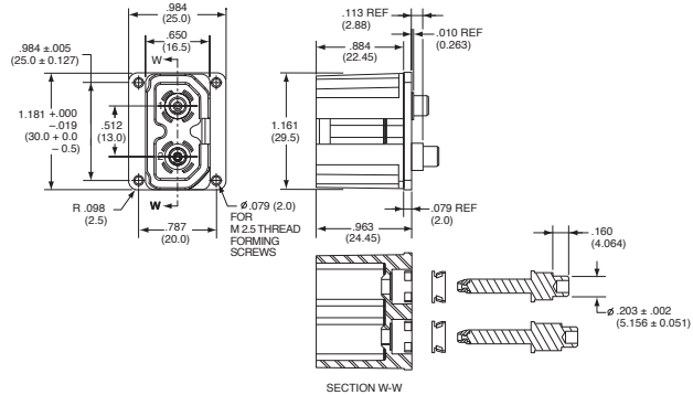
10-638977-000 PCB Tail Receptacle
